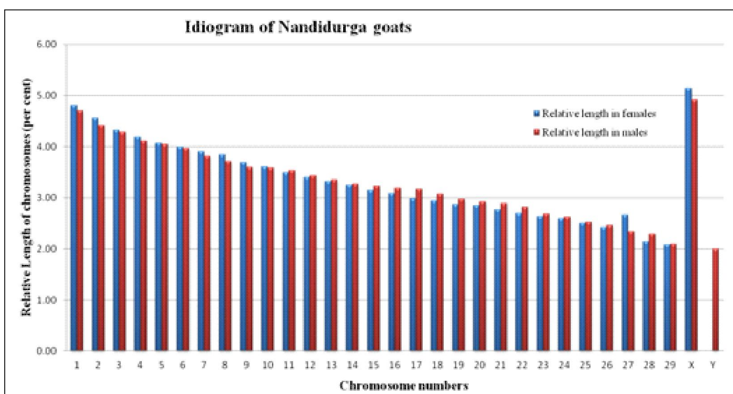
Fig 3: Idiogram based on relative length of chromosomes of Nandidurga goats.
