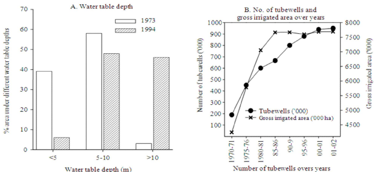
FIG. 3: Water utilization: (A) Change in percentage of area under different water table depths from 1973 to 1994. (B) Increase in no. of tubewells and gross irrigated area over time. Data source: SAP(2007).
