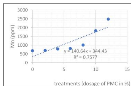
Fig 13: Correlation of Mn with dosage of PMC.
