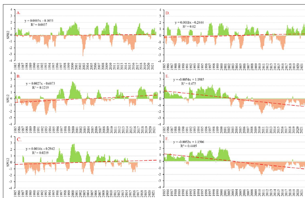
Fig 5: Temporal evolution of drought trends for 12-months drought timescale (SPI-12) at rainfall observation stations A) Chau Doc, B) Long Xuyen, C) Kien Luong, D) Rach Gia, E) Ha Tien and F) Tan Hiep during the period of (1984-2022).
