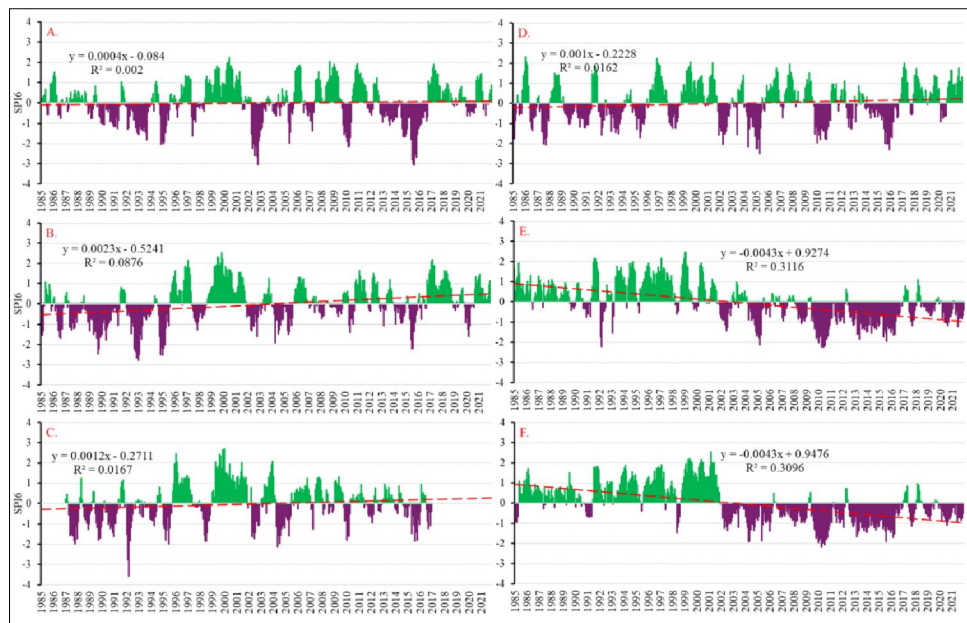
Fig 4: Temporal evolution of drought trends for 6-months drought timescale (SPI-6) at rainfall observation stations A) Chau Doc, B) Long Xuyen, C) Kien Luong, D) Rach Gia, E) Ha Tien and F) Tan Hiep during the period of (1984-2022).
