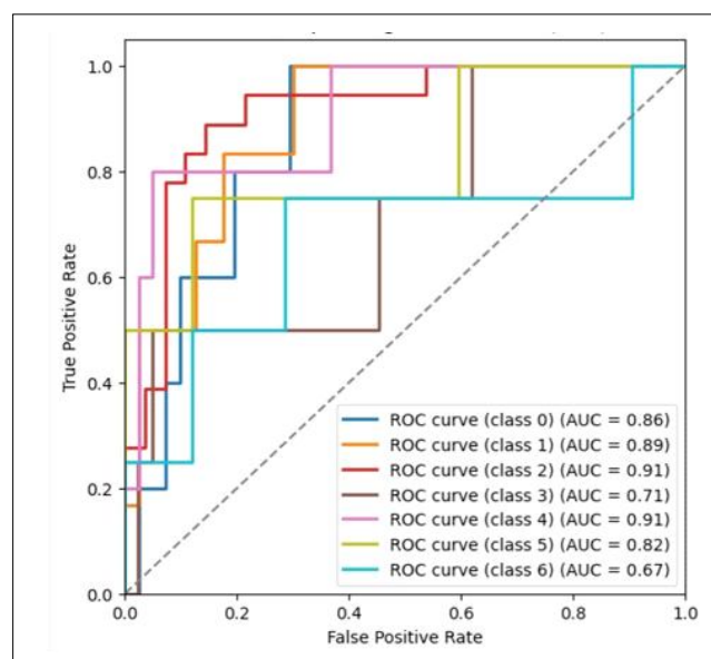
Fig 4: ROC-AUC curve.
