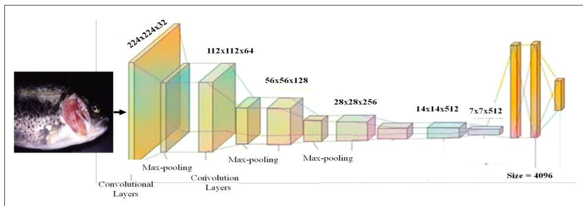
Fig 1: VGGNet-19 modal.
