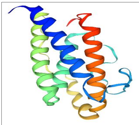
Fig 4: Three-dimensional structure prediction result of leptin protein in E. miletus .
