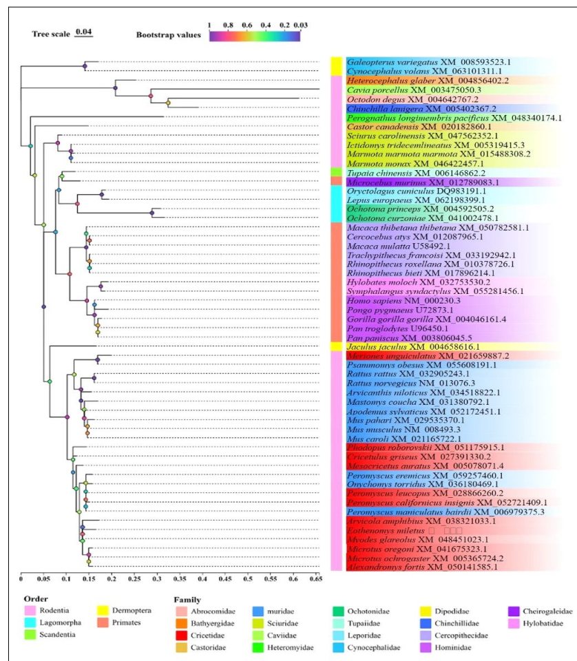
Fig 6: Phylogenetic tree of 56 mammalian leptin genes.
