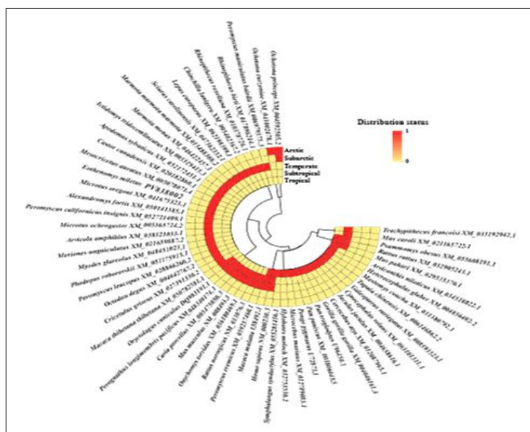
Fig 7: Clustering heat map of the distribution of 56 species in each temperature zone.
