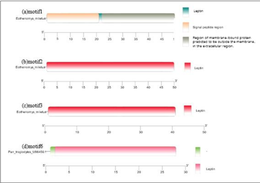
Fig 9: Functional annotation results of each conserved motif.
