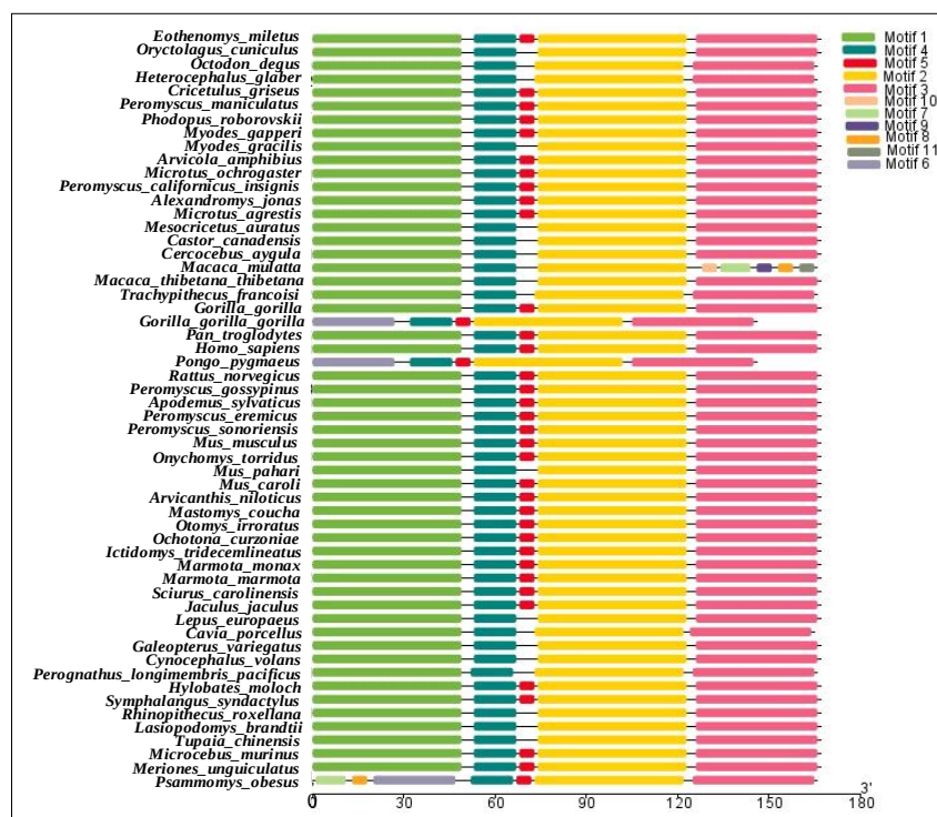
Fig 8: Results of conserved motif determination of 56 leptin gene sequences.
