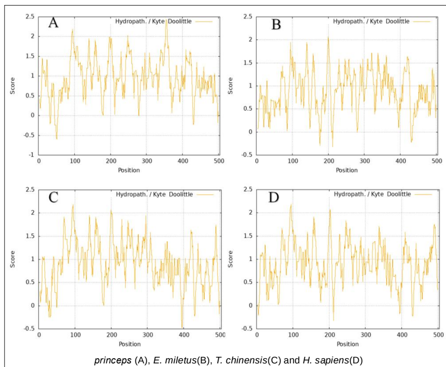
Fig 5: Prediction results of leptin affinity/hydrophobicity of O.
