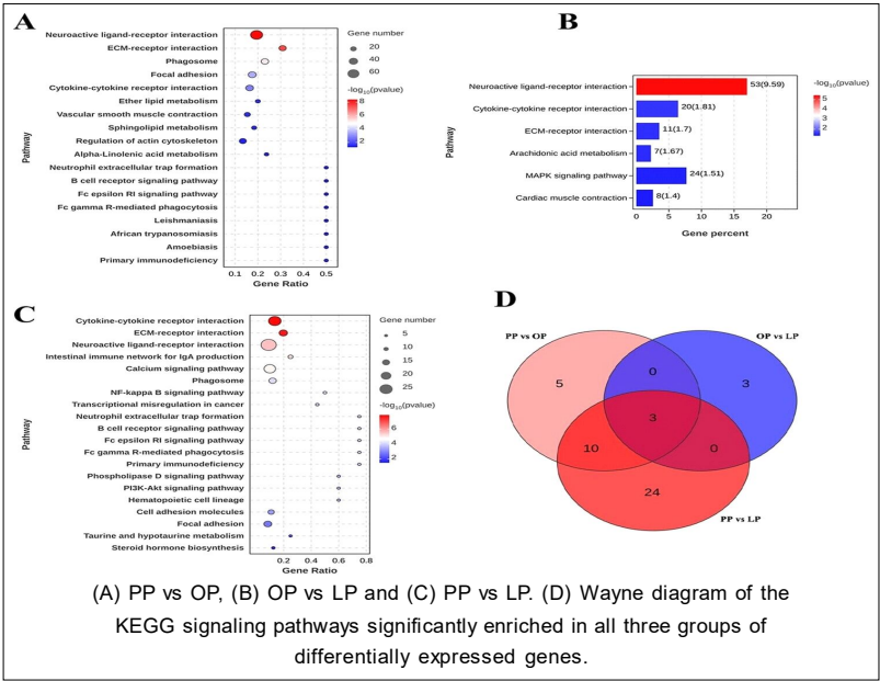
Fig 3: The KEGG signaling pathways of differentially expressed genes significantly enriched in.
