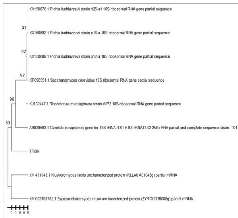
Fig 4: Phylogenetic tree.
