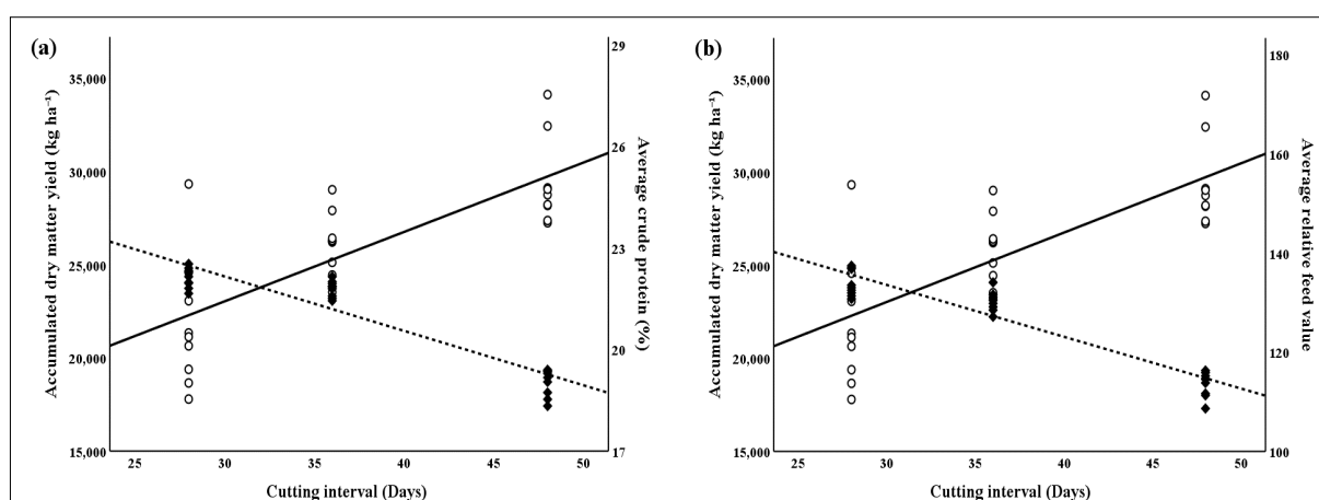
Fig 3: The relationship between accumulated dry matter yield and average crude protein content (a) and relative feed value (b) of alfalfa by cutting intervals during production years. The circular symbol (o) and straight line are accumulated dry matter yield. The diamond symbol (♦) and dotted line are average crude protein content and relative feed value.
