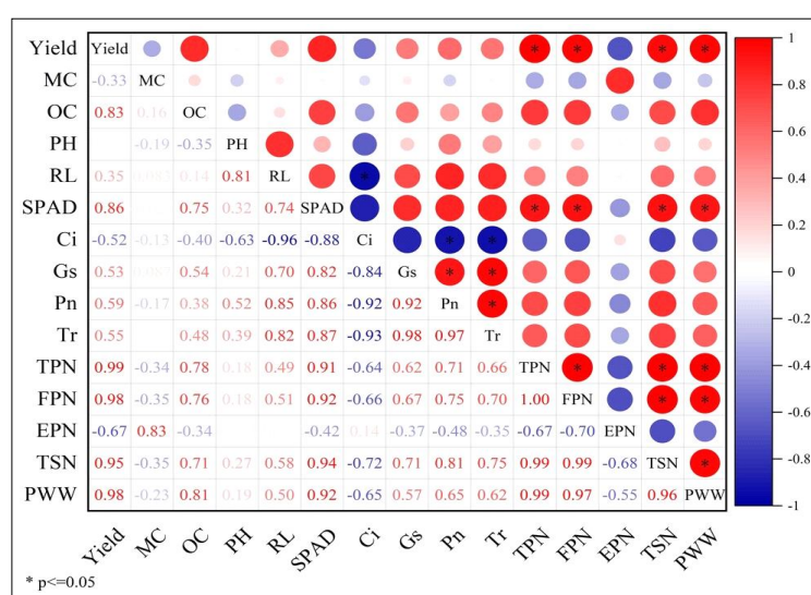
Fig 3: Correlation analysis among agronomic traits of soybean under drought stress.
