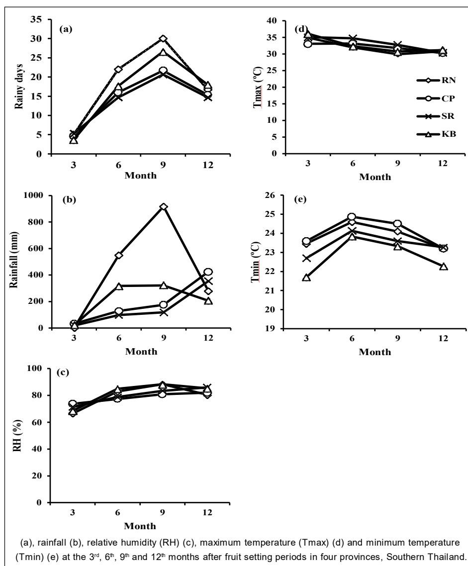
Fig 1: Variations in the rainy days.
