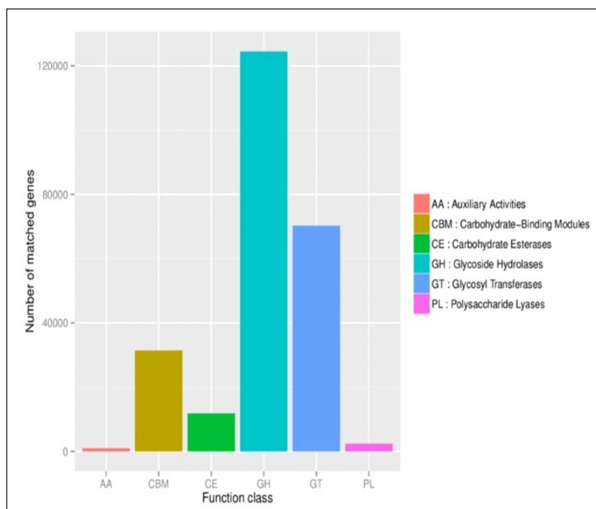
Fig 10: CAZy analysis for number of unigenes.
