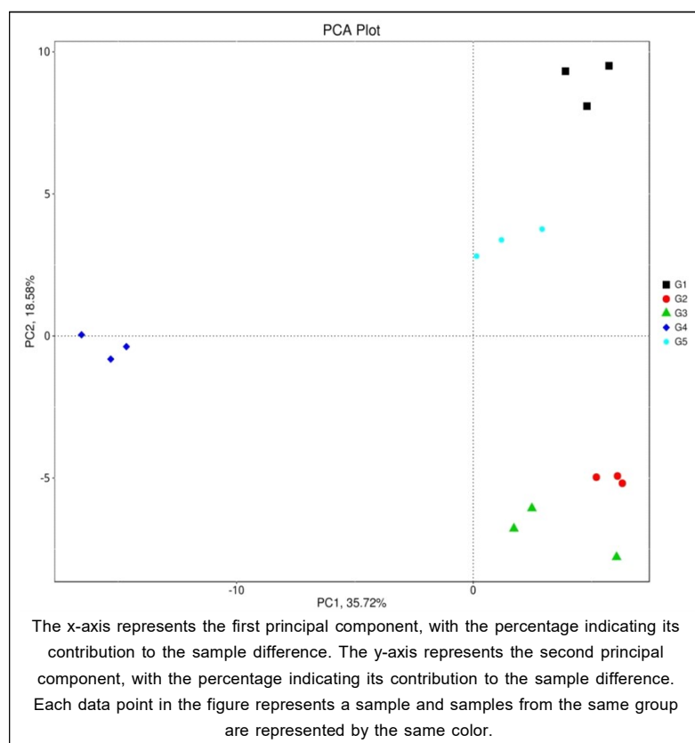
Fig 3: Principal component analysis (PCA) results at phylum.
