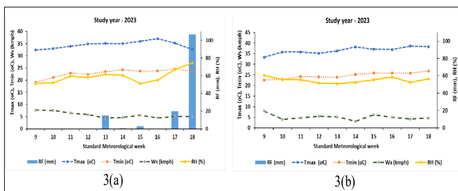
Fig 3: Observed weather during the study period Jan-May 2023(a) and 2024(b).
