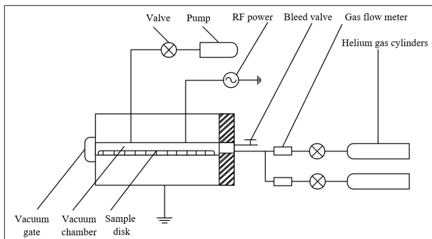
Fig 1: Schematic of low temperature plasma test platform.
