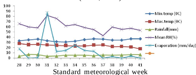
FIG 1: Mean weekly meteorological data for crop season (kharif, 2008)
